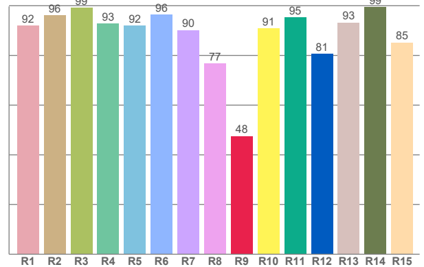
CRI: 91.9 (R1-R8)
