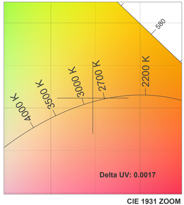
CRI: 91.9 (R1-R8)
